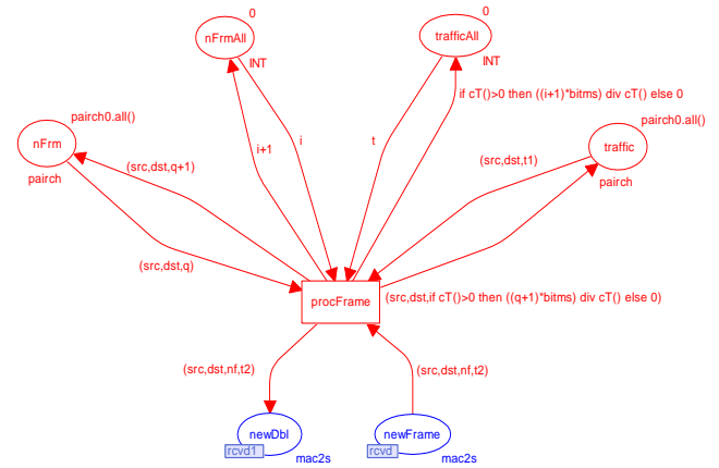
Fig. 4. Measuring fragment for traffic evaluation
