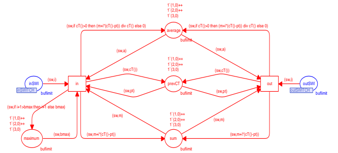
Fig. 6. Measuring fragment for switch buffer size evaluation
